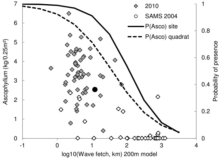
Fig. 5. The relationship between average wet weight of Ascophyllum nodosum plants in 0.25m 2 quadrats and wave exposure, expressed as the logarithm to base 10 of total wave fetch in km. Weight of plants is shown against the left-hand axis and the probabilities of presence of Ascophyllum at sites (solid line) and in each quadrat (dashed line) are plotted against the right hand axis.
