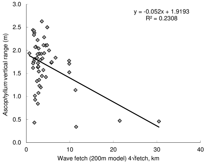
Fig. 6. The relationship between Ascophyllum vertical range and wave exposure.
